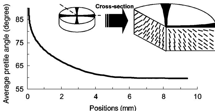
FIGURE 9 Simulated pretilt angle distribution of the AS-SPNLC cell.
