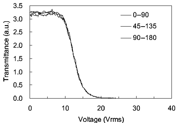
FIGURE 7 Voltage-dependent transmittance of the AS-SPNLC cell. d = 9 \mu\text{m} and \lambda = 633 \text{ nm} .
