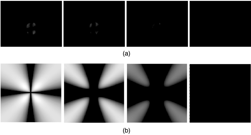
FIGURE 11 (a) Experimental results when a voltage is applied to the AS-SPNLC, and (b) simulated results.
