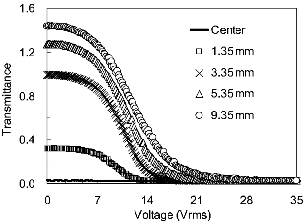
FIGURE 10 Measured V-T curves at different positions of the AS-SPNLC cell.
