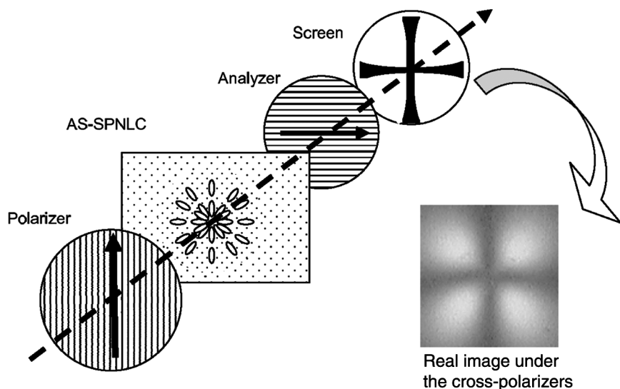
FIGURE 2 SPNLC structure observed under crossed polarizers.
