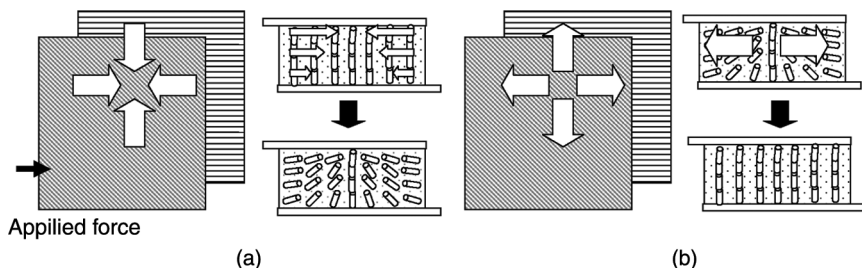
FIGURE 4 Illustration of external force and movement of the liquid crystal directors (a) initial state, and (b) relaxed state.
