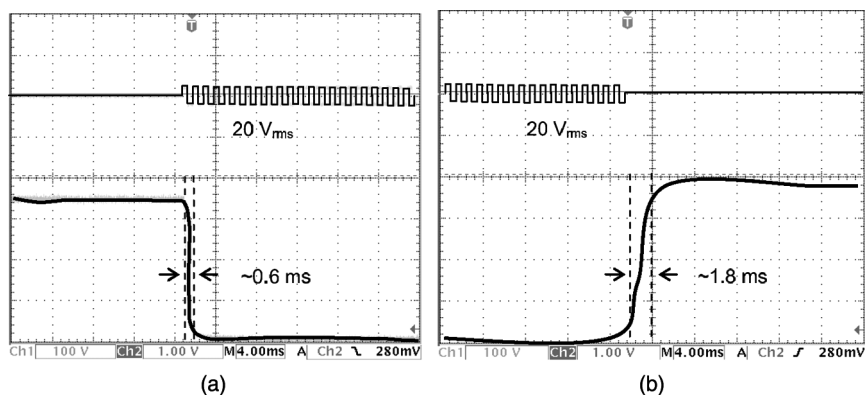
FIGURE 8 Optical response time of a 9\text{-}\mu\text{m} AS-SPNLC: (a) rise time, and (b) decay time.
